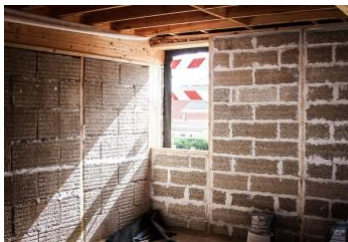
Figure 3. Hemp blocks for interior and exterior wall.
